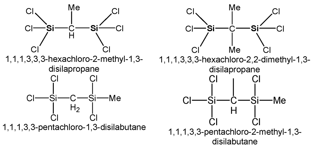
[0036] Table 1. Silicon precursors having one Si-C-Si linkage
