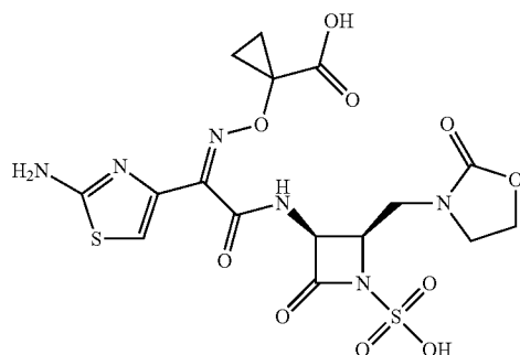
[0428] Beta-Lactam 5 (LYS228):
