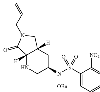
Step 2: N-((3R,4aS,7aS)-6-allyl-7-oxooctahydro-1H-pyrrolo[3,4-b]pyridin-3-yl)-N-(benzyloxy)-2-nitrobenzenesulfonamide
