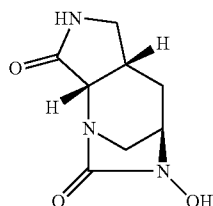
Step 3: (4R,5aS,8aS)-3-hydroxyhexahydro-2H-1,4-methanopyrrolo[3,4-d][1,3]diazepine-2,8(8aH)-dione
