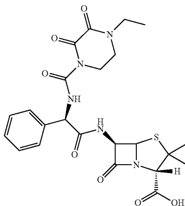
[0428] Beta-Lactam 5 (LYS228):
